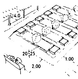
④ Simple rows of graves with prescribed planting (proposed by H. Hartwig)
